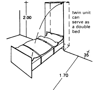
16 Top-hinged folding bed
